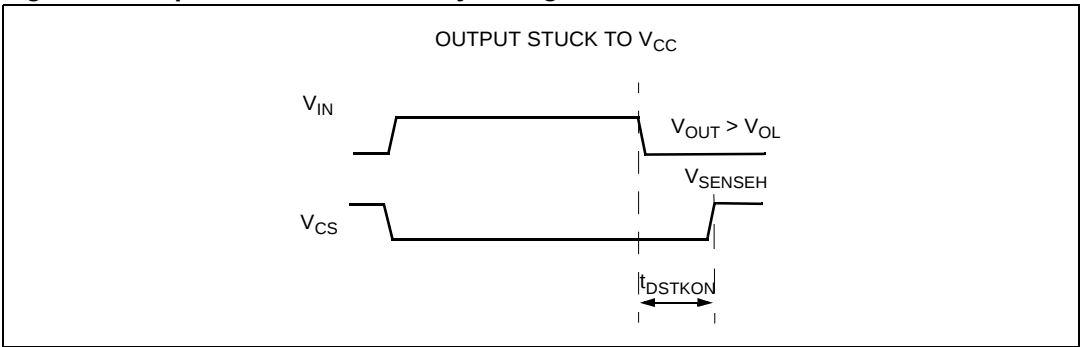
Figure 5. Open load off-state delay timing
