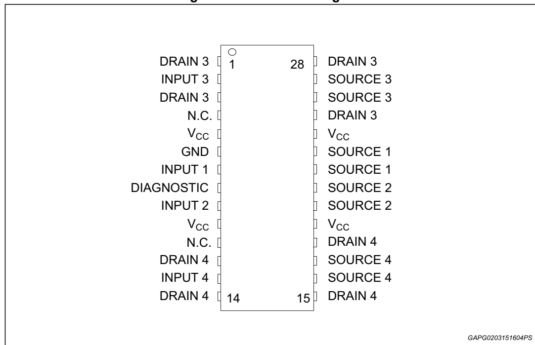
Figure 2. Connection diagram
