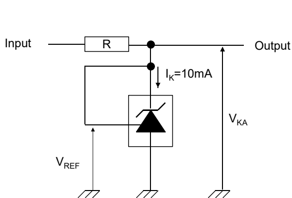
Figure 7. Test circuit for V_{KA} = V_{ref}
