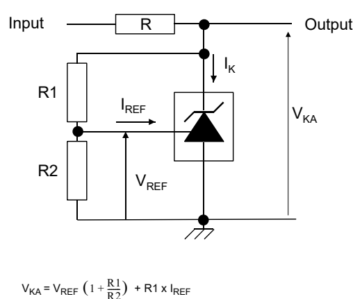
Figure 8. Test circuit for programming mode
