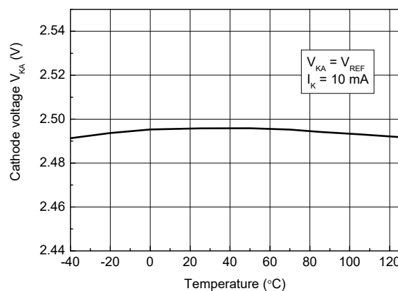
Figure 12. Reference voltage vs. temperature
