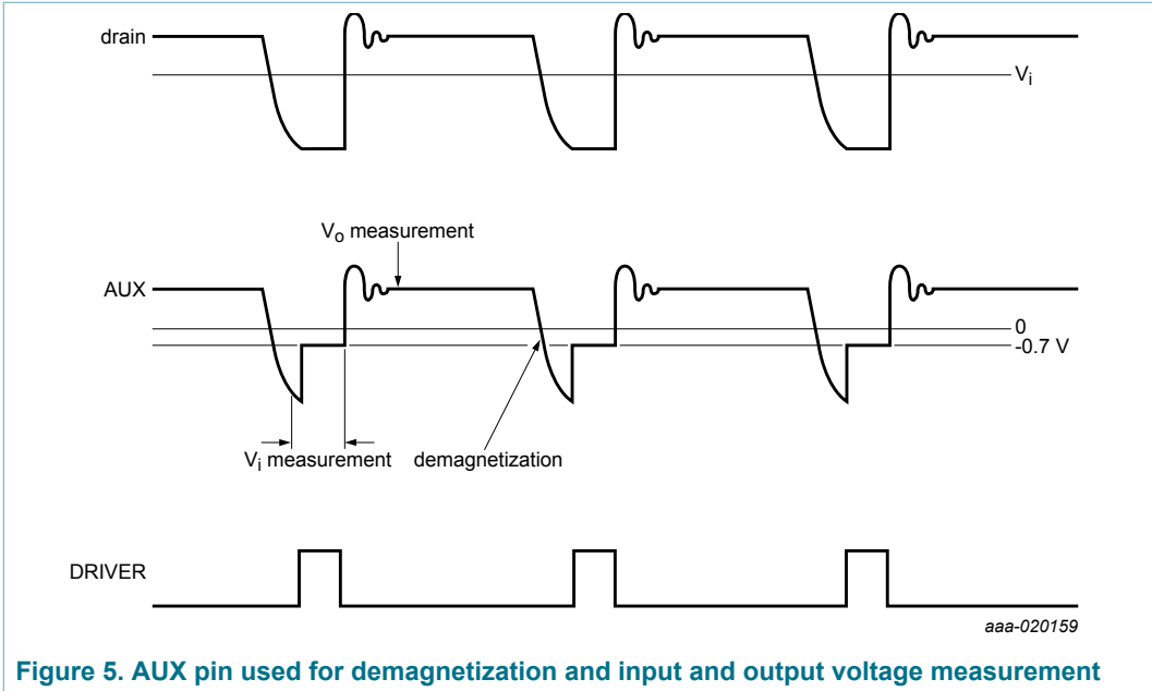
When the external MOSFET is switched on, the voltage at the auxiliary windings reflects the input voltage. The AUX pin is clamped to -0.7\text{ V} . The output current is a measure of the input voltage. This current value is internally used to set the overpower limit on V_{\text{sense(ipk)}} . The demagnetization and output voltages are measured as a voltage on the AUX pin. In this way, the input voltage measurement and OVP can be adjusted independently.
