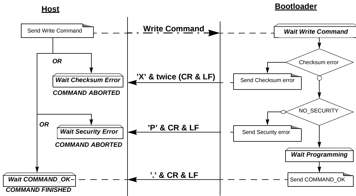
Figure 27. Write/Program Flow
