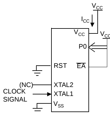
Figure 34. I_{CC} Test Condition, Idle Mode
