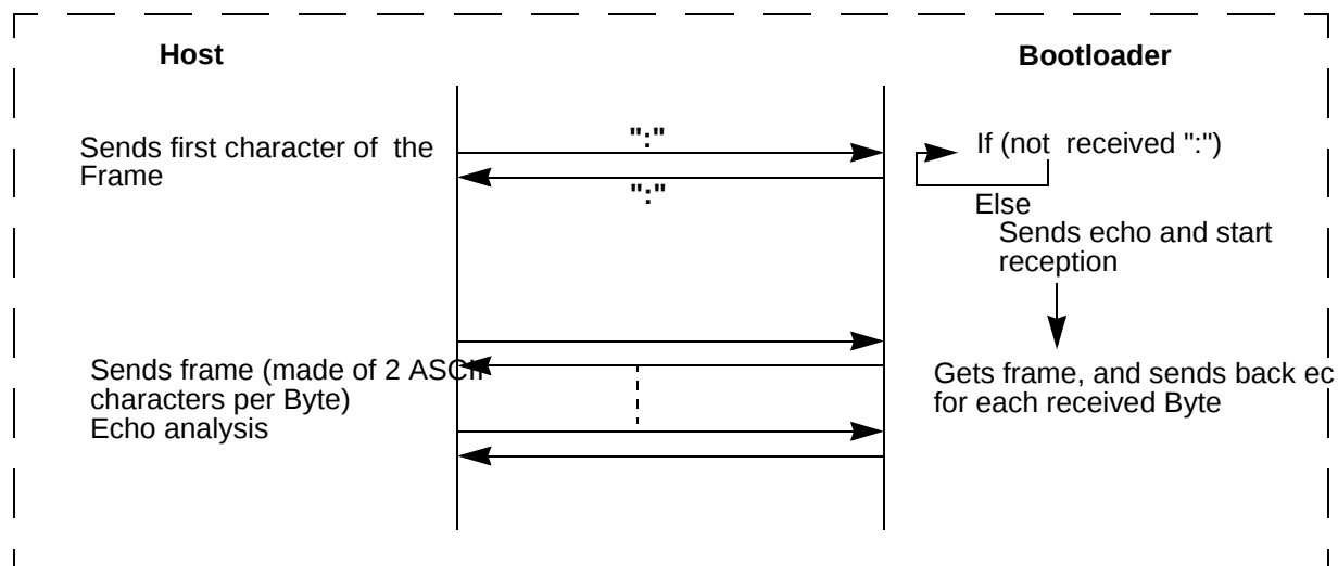
Figure 26. Command Flow
