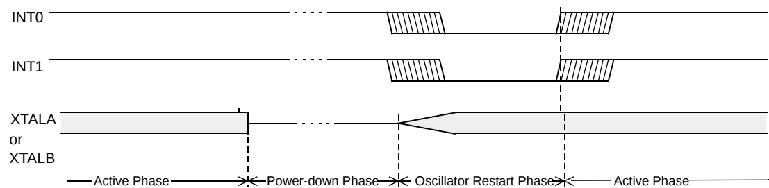
Figure 19. Power-down Exit Waveform
