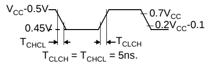
Figure 35. I_{CC} Test Condition, Power-Down Mode
