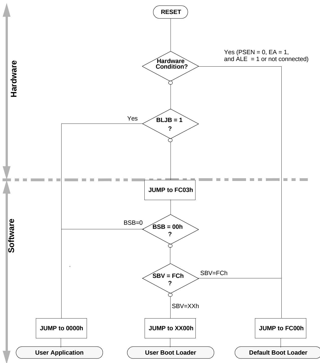
Figure 24. Bootloader Process
