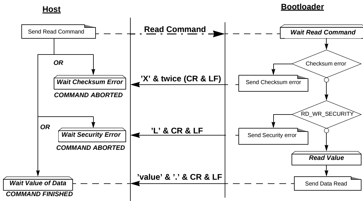
Figure 30. Read Flow
