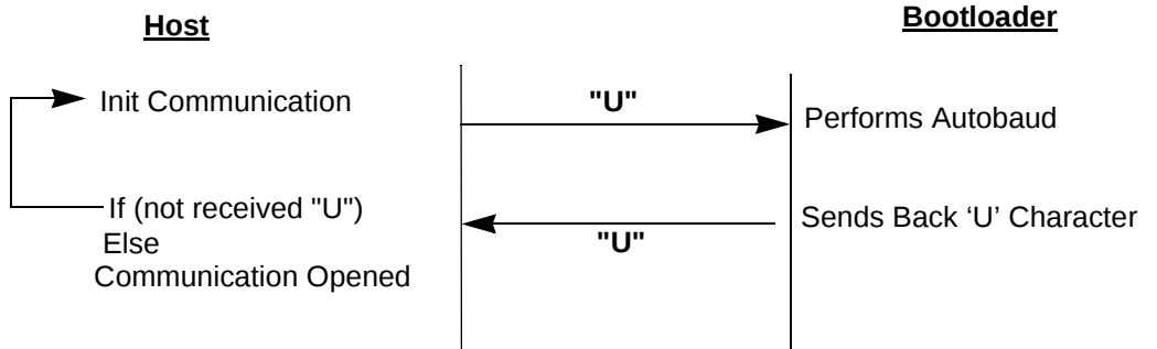
Figure 25. Initialization
