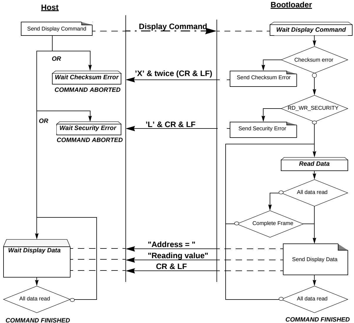
Figure 29. Display Flow
