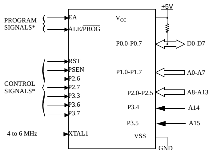
Figure 31. Set-Up Modes Configuration
