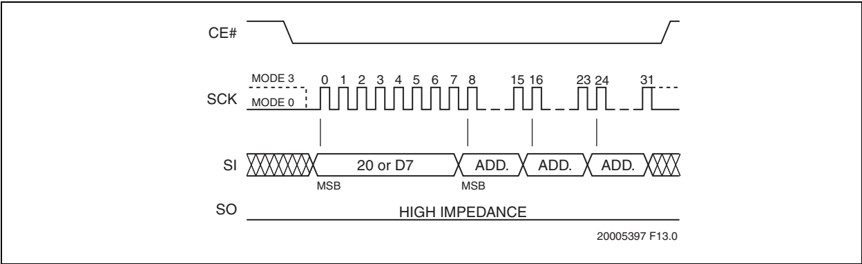
FIGURE 5-6: SECTOR-ERASE SEQUENCE
