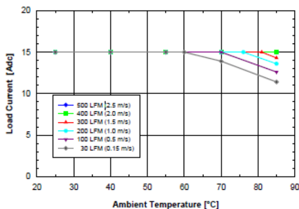
Fig. 2.OV.1: Available load current vs. ambient temperature and airflow rates for SQ48T15020 converter with D height pins mounted vertically with V_{in} = 48\text{ V} , air flowing from pin 3 to pin 1, and maximum FET temperature \leq 120^\circ\text{C} .
