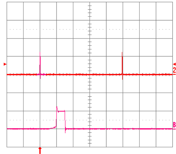
Fig. 2.5V.18: Load current (top trace, 20\text{ A/div.} , 20\text{ ms/div.} ) into a 10\text{ m}\Omega short circuit during restart, at V_{in} = 48\text{ V} . Bottom trace ( 20\text{ A/div.} , 1\text{ ms/div.} ) is an expansion of the on-time portion of the top trace.
