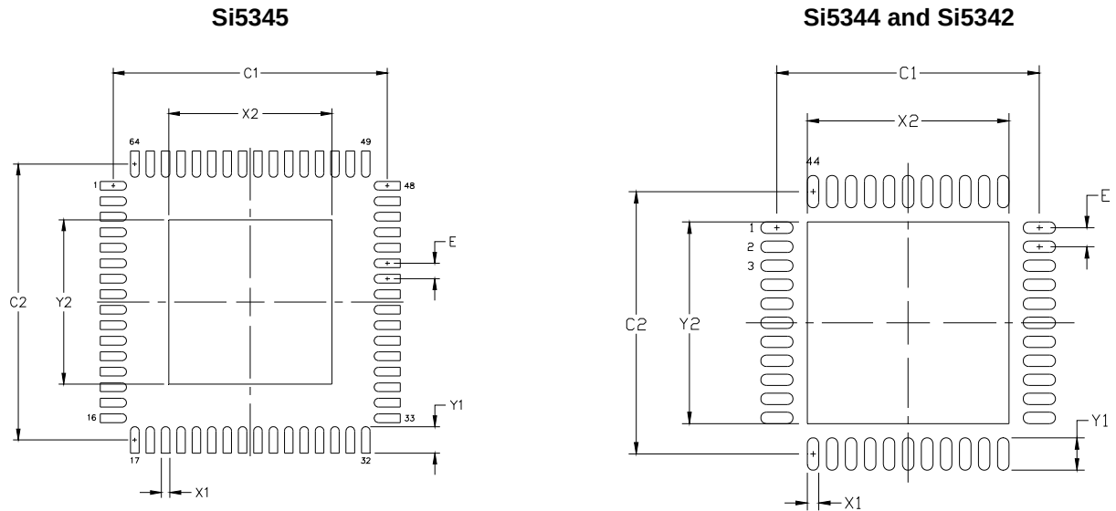
Figure 25. PCB Land Pattern
