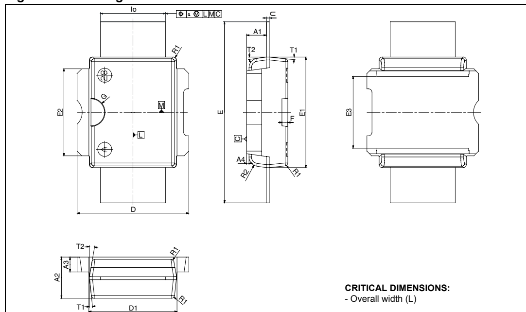
Figure 22. Package dimensions
