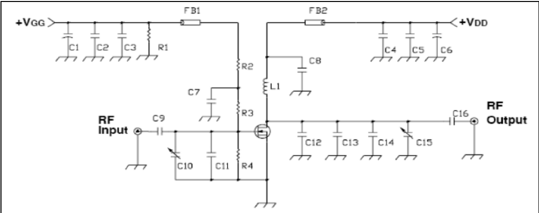
Figure 20. 175 MHz test circuit schematic (engineering)
