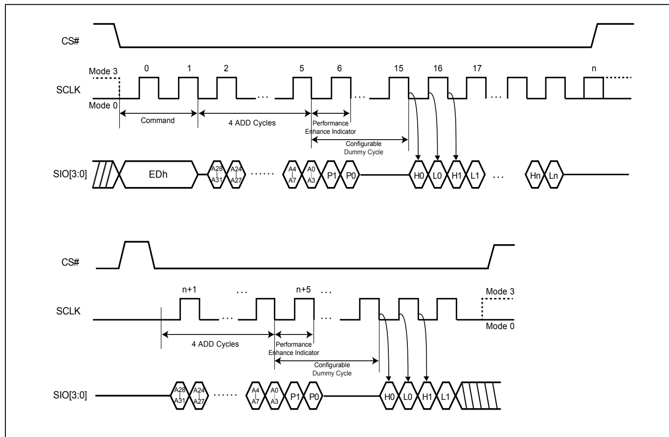
Figure 45. 4 x I/O DT Read Performance Enhance Mode Sequence (QPI Mode)
