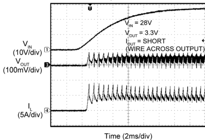
Power Up into Short Circuit
