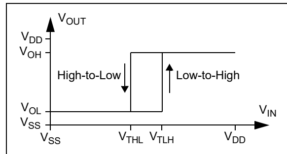
FIGURE 4-5: Hysteresis Diagram for the Noninverting Circuit.
