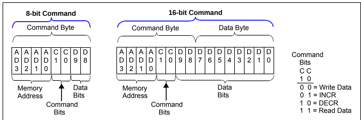
FIGURE 7-1: General SPI Command Formats.
