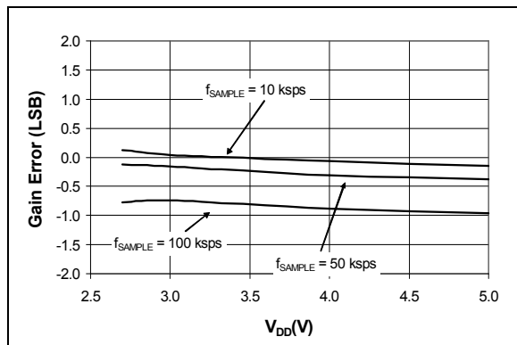
FIGURE 2-15: Gain Error vs. V_{DD} .
