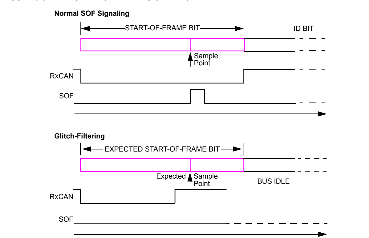
FIGURE 3-5: START-OF-FRAME SIGNALING
