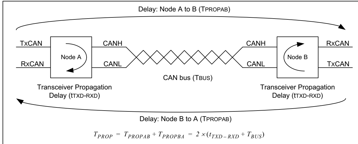
FIGURE 3-11: PROPAGATION DELAY
