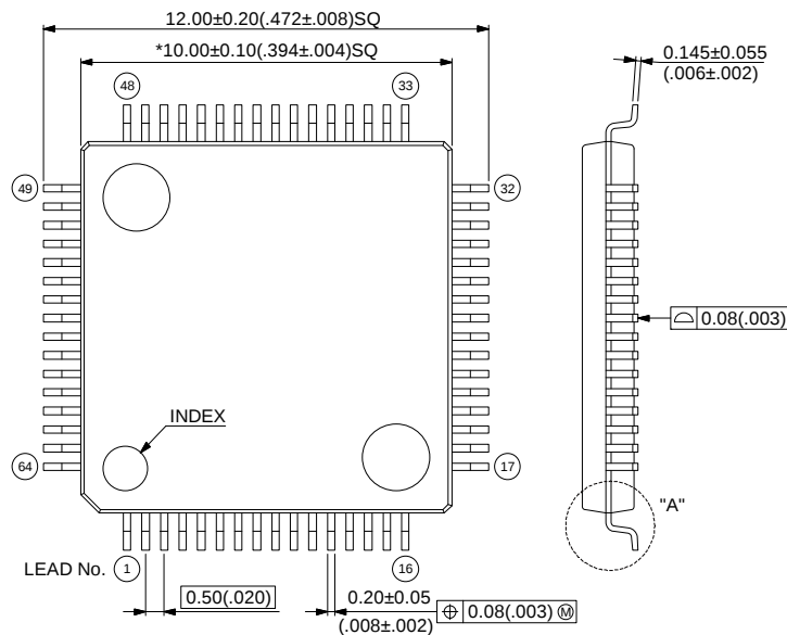
64-pin plastic LQFP (FPT-64P-M24)
