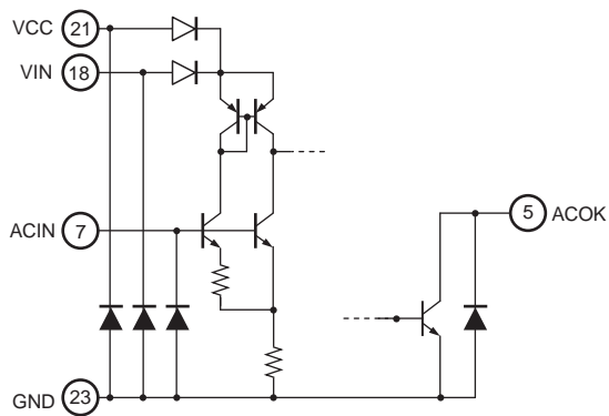
<Bias voltage block>
