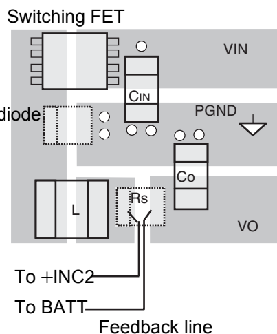
Switching system part arrangement example
