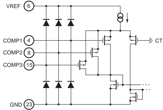
<AC adapter detection block>
