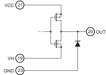
<Output block>
