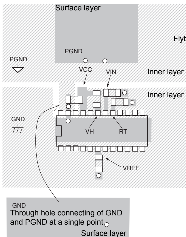
GND wiring example
