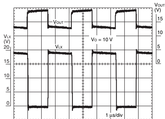
Switching waveform (Constant current mode)
