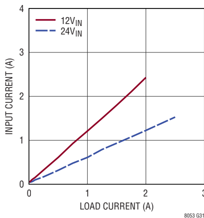
LTM8053 Input vs Load Current V_{OUT} = -12\text{V} , BIAS tied to LTM8053 GND
