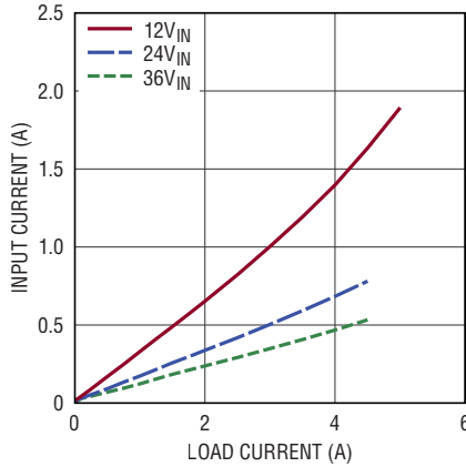
LTM8053 Input vs Load Current V_{OUT} = -3.3\text{V} , BIAS tied to LTM8053 GND
