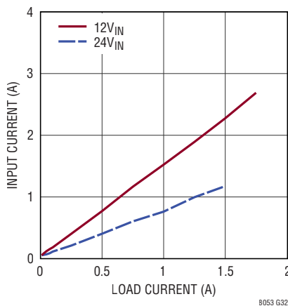
LTM8053 Input vs Load Current V_{OUT} = -15\text{V} , BIAS Tied to LTM8053 GND
