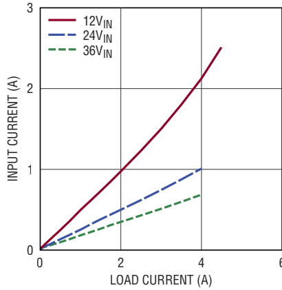
LTM8053 Input vs Load Current V_{OUT} = -5\text{V} , BIAS Tied to LTM8053 GND
