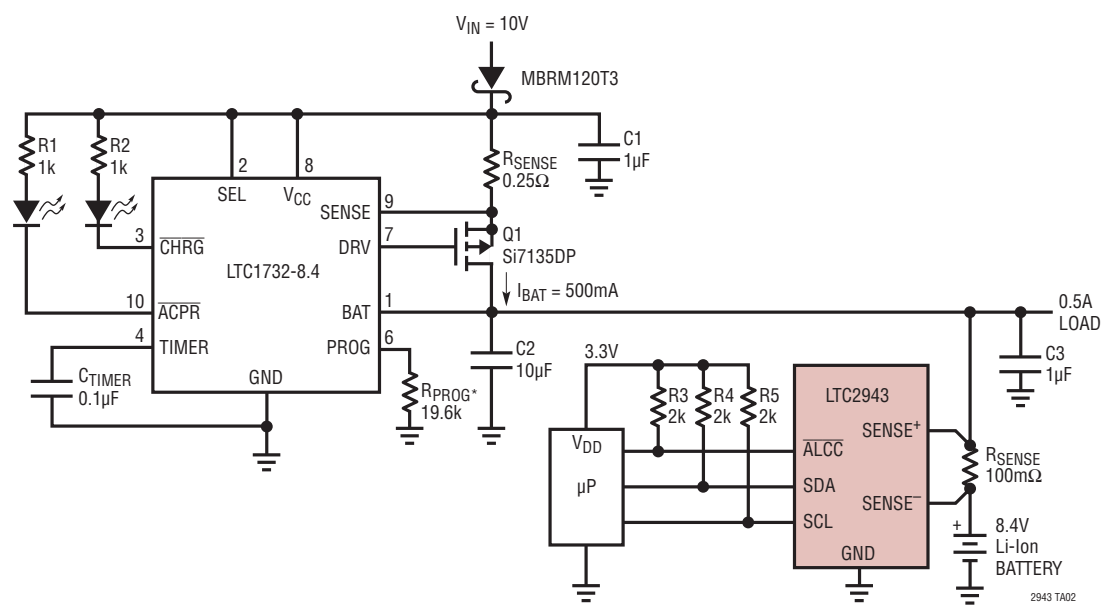
2-Cell 8.4V Linear Charger and Battery Gas Gauge
