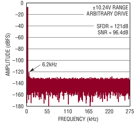
32k Point Arbitrary Two-Tone FFT f_{SAMPL} = 550\text{ksps} , IN^+ = -7\text{dBFS } 2\text{kHz} Sine, IN^- = -7\text{dBFS } 3.1\text{kHz} Sine
