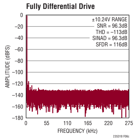
Figure 6c. IN^+/IN^- = -1\text{dBFS} 2kHz Fully Differential Sine, V_{\text{CM}} = 0\text{V} , 32k Point FFT, f_{\text{SAMPL}} = 550\text{ksps} . Circuit Shown in Figure 6a
