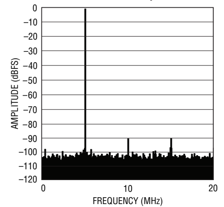
LTC2264-14: 8k Point FFT, f_{IN} = 5\text{MHz} , -1dBFS, 40Msps
