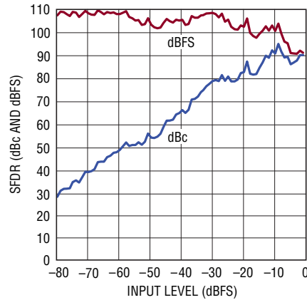
LTC2265-14: SFDR vs Input Level, f_{IN} = 70\text{MHz} , 2V Range, 65Msps
