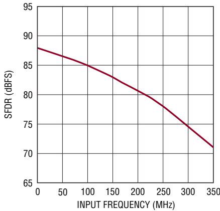
LTC2265-14: SFDR vs Input Frequency, -1dBFS, 2V Range, 65Msps
