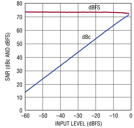
LTC2265-14: SNR vs Input Level, f_{IN} = 70\text{MHz} , 2V Range, 65Msps
