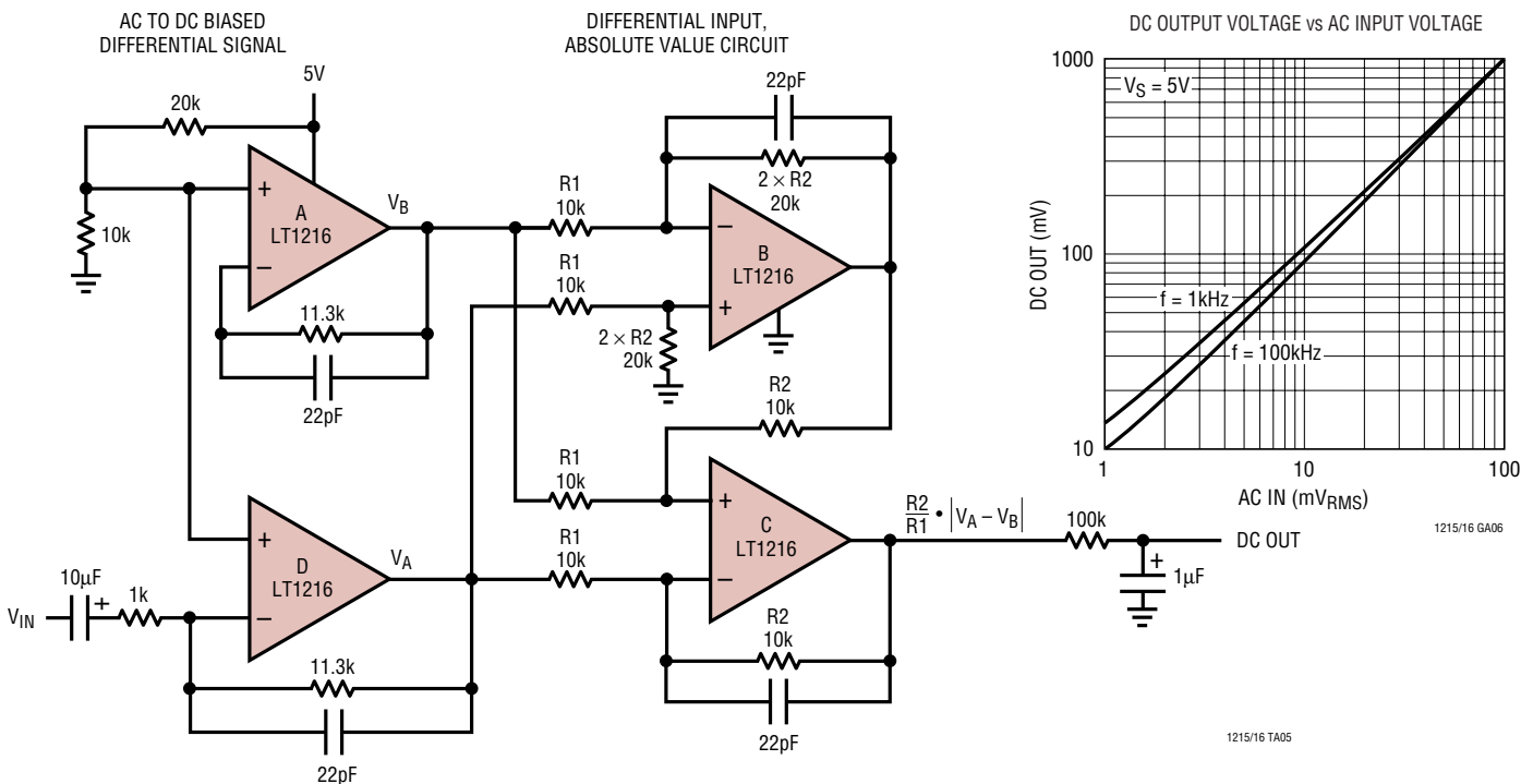
Single Supply, AC Coupled Input, RMS Calibrated, Average Detector
