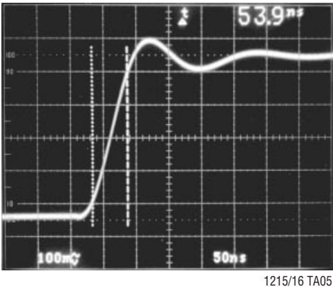
TRANSIENT RESPONSE
