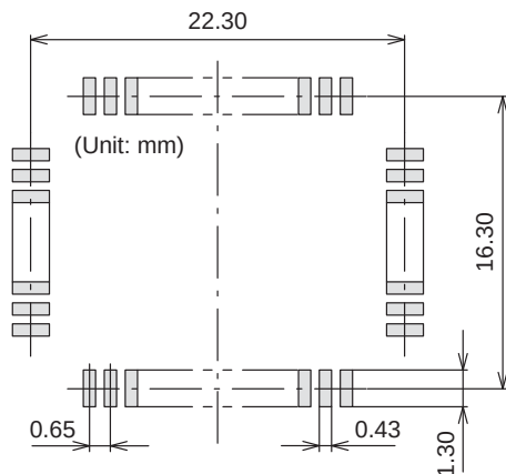
SOLDERING FOOTPRINT*
