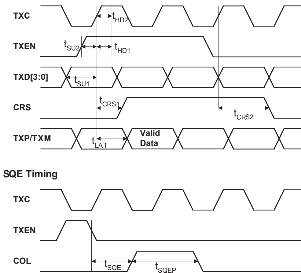
Figure 4. 10BaseT MII Transmit Timing
