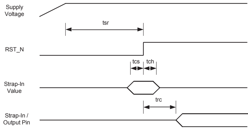
Figure 9. Reset Timing
