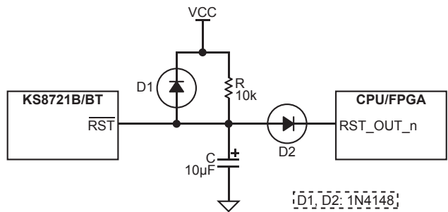
Figure 10. Recommended Reset Circuit.
