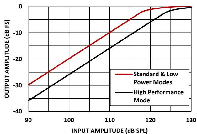
Figure 7. Linearity
