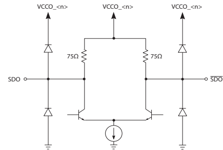
Figure 3-2: SDO0/ \overline{SDO0} and SDO1/ \overline{SDO1}
