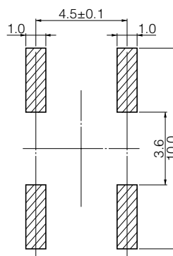
PWB land pattern for reference
