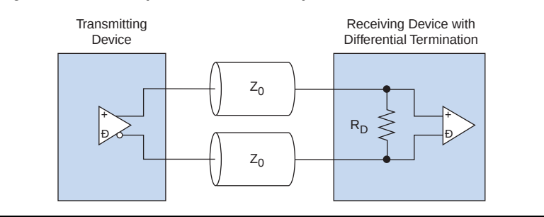
Figure 4–70. LVDS Input Differential On-Chip Termination
