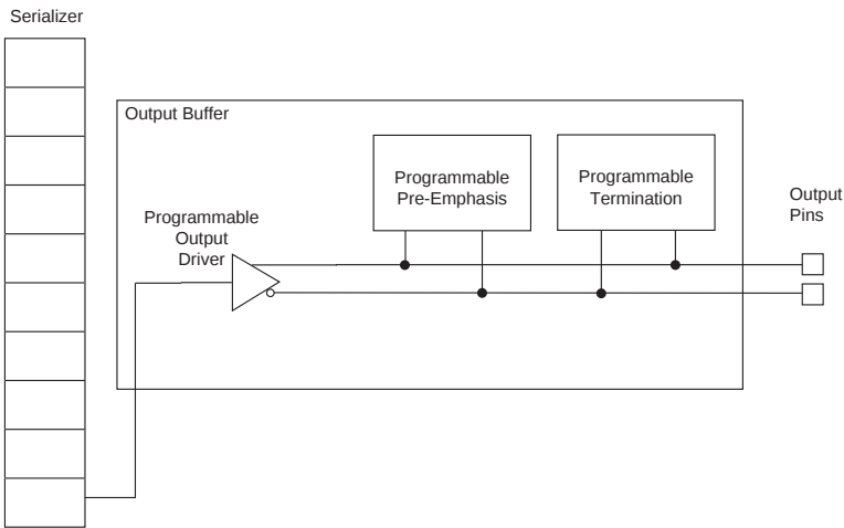
Figure 2–6. Output Buffer
