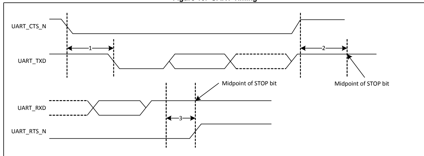
Figure 10. UART Timing
