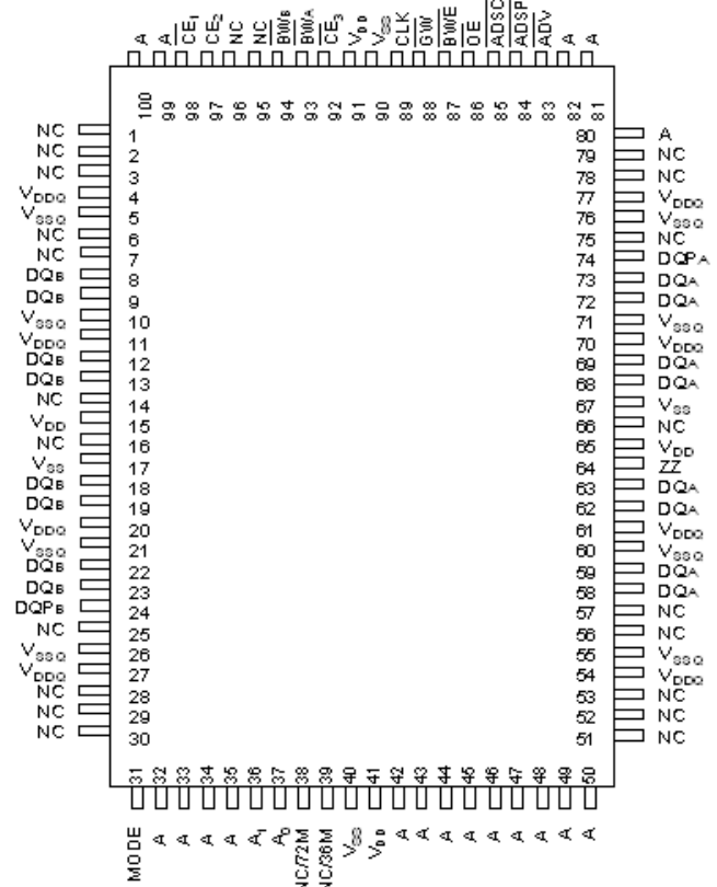
CY7C1383KV33/CY7C1383KVE33 (1M × 18)
