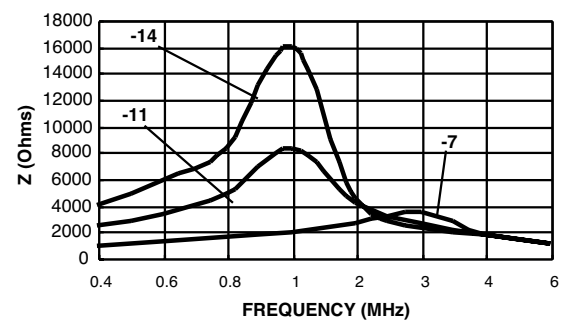
Impedance CMS2 - 7,11, & 14
