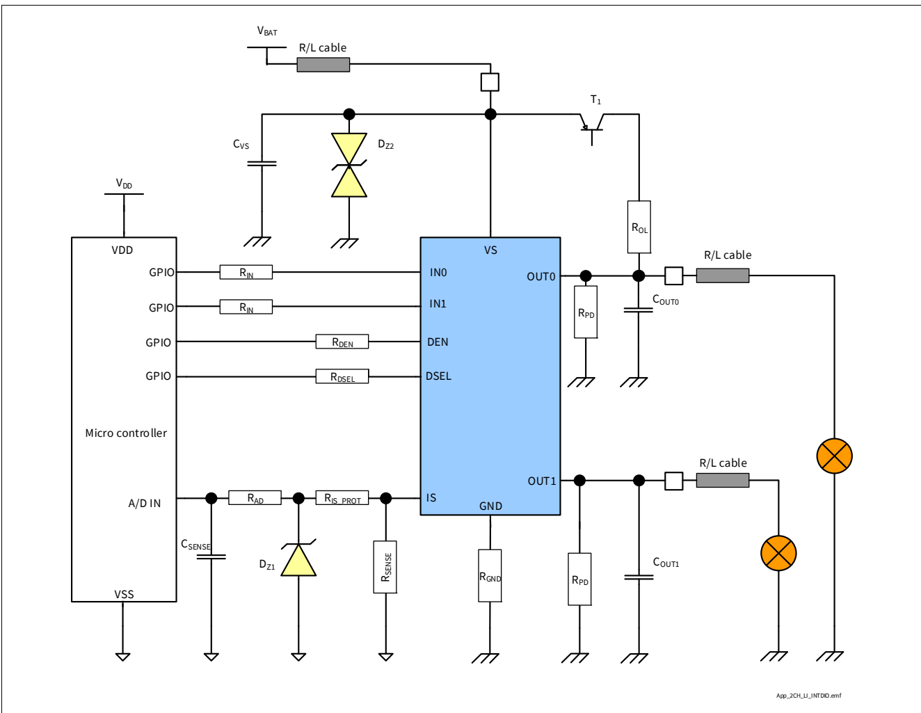
Figure 43 BTS7030-2EPA Application Diagram
