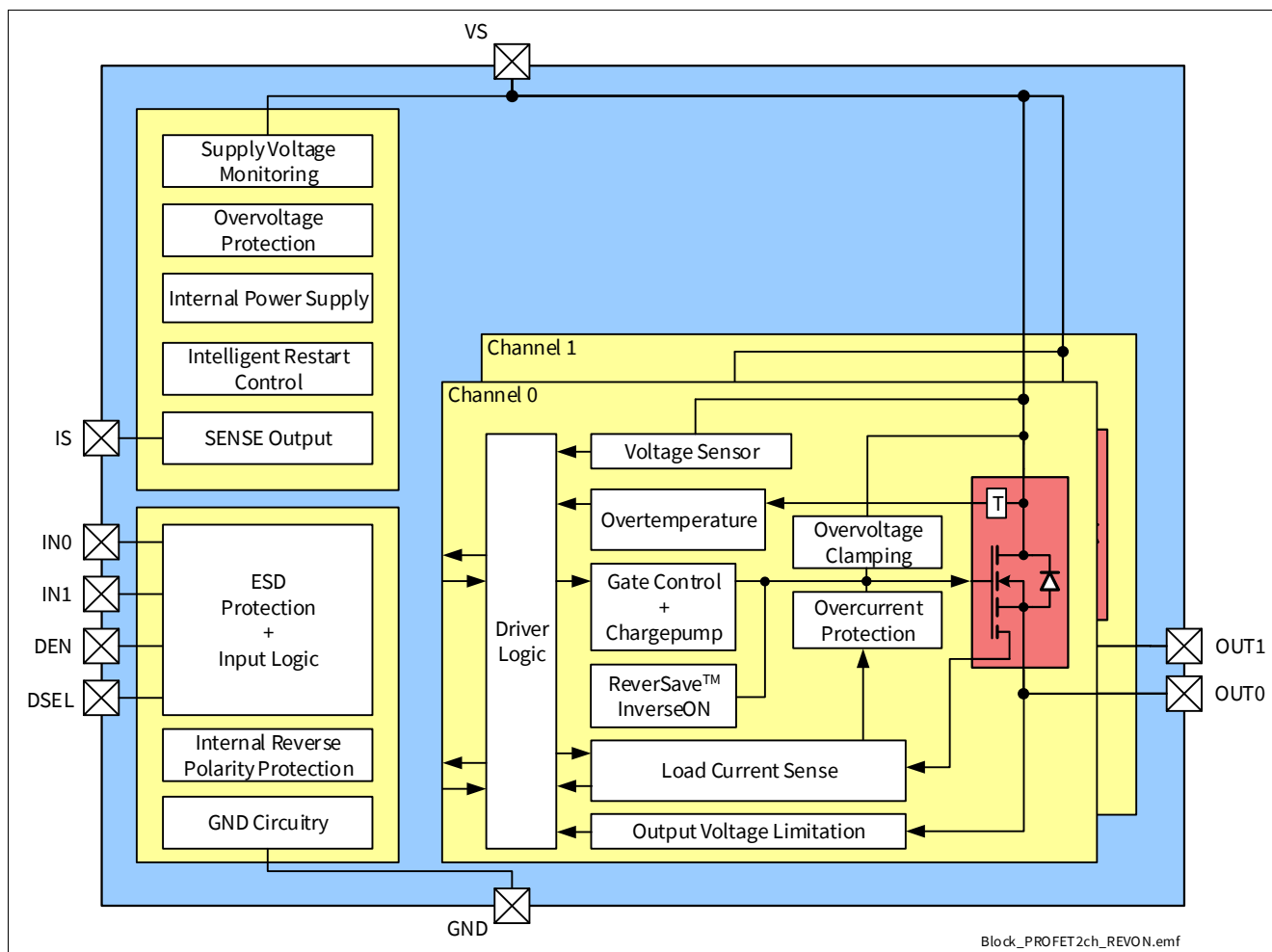
Figure 2 Block Diagram of BTS7030-2EPA
