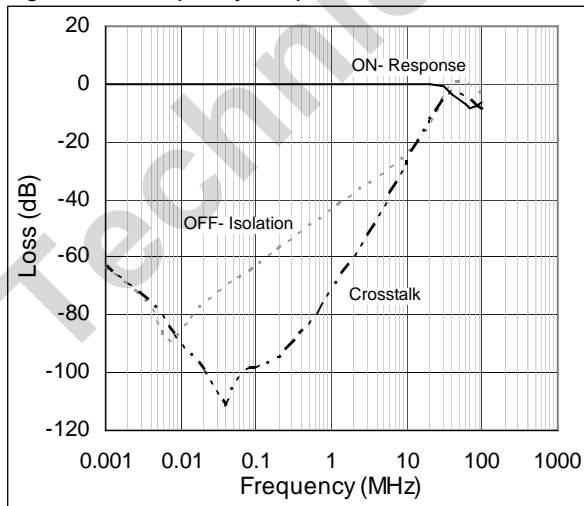
Figure 14. Frequency Response
