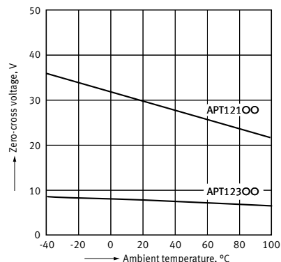
8. Zero-cross voltage vs. ambient temperature characteristics
