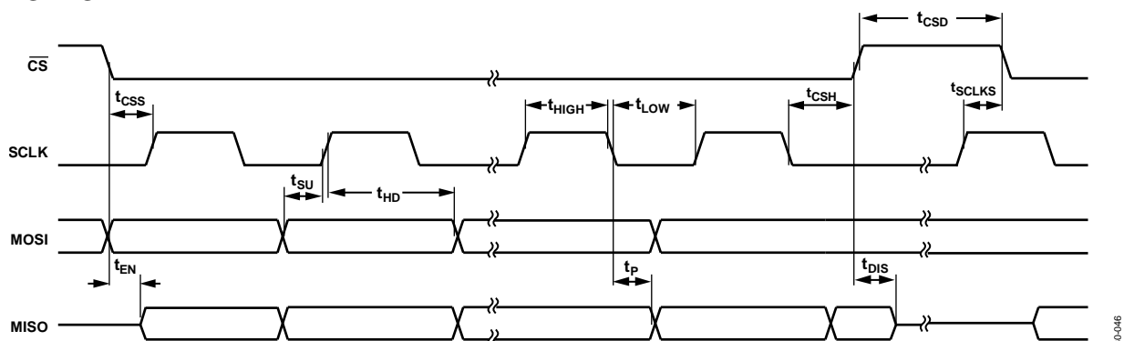
Figure 39. SPI Timing Diagram
