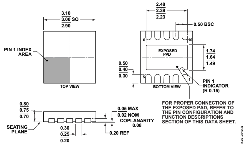
Figure 32. 10-Lead Lead Frame Chip Scale Package [LFCSP_WD] 3 mm x 3 mm Body, Very Very Thin, Dual Lead (CP-10-9)
