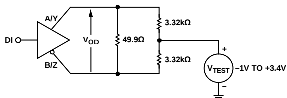
Figure 19. Driver Voltage Measurement over Common-Mode Range
