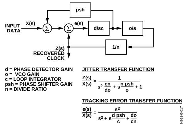
Figure 17. ADN2813 PLL/DLL Architecture
