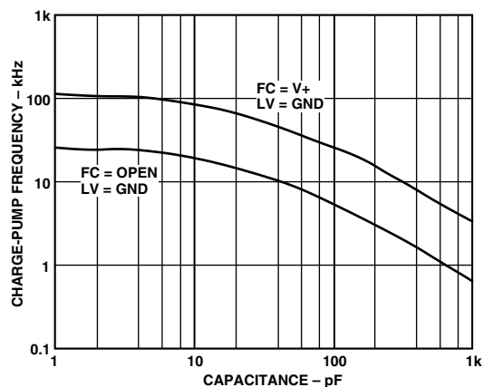
TPC 11. Charge-Pump Frequency vs. External Capacitance
