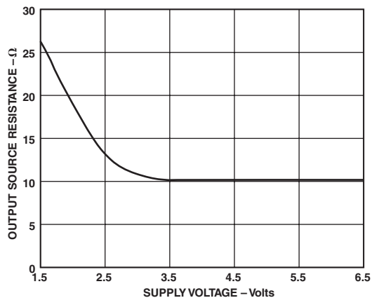
TPC 8. Output Source Resistance vs. Supply Voltage
