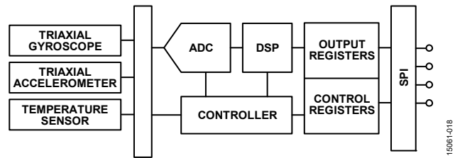
Figure 26. Basic Operation
