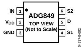
Figure 2. Pin Configuration
