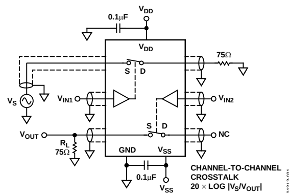
Figure 21. Channel-to-Channel Crosstalk
