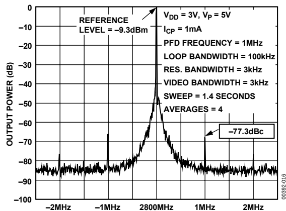
Figure 16. ADF4118 Reference Spurs (2800 MHz, 1 MHz, 100 kHz)
