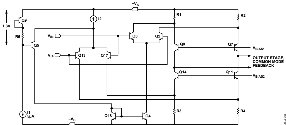
Figure 63. Simplified Schematic
