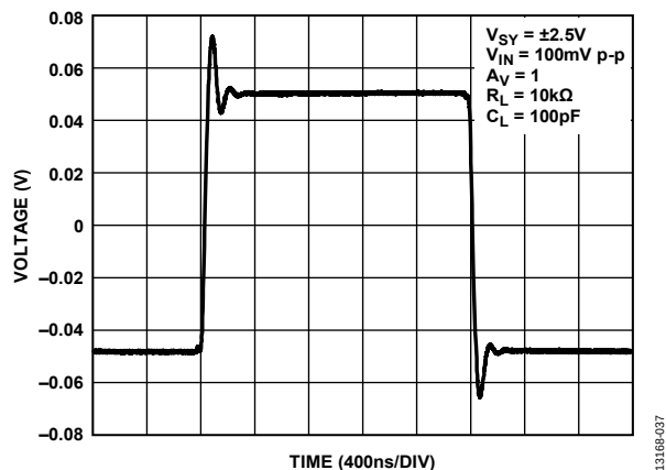
Figure 39. Small Signal Transient Response, V_{SY} = \pm 2.5V
