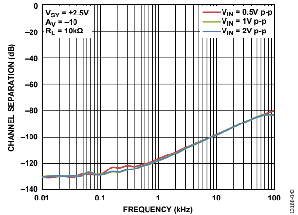
Figure 45. Channel Separation vs. Frequency, V_{SY} = \pm 2.5\text{ V}
