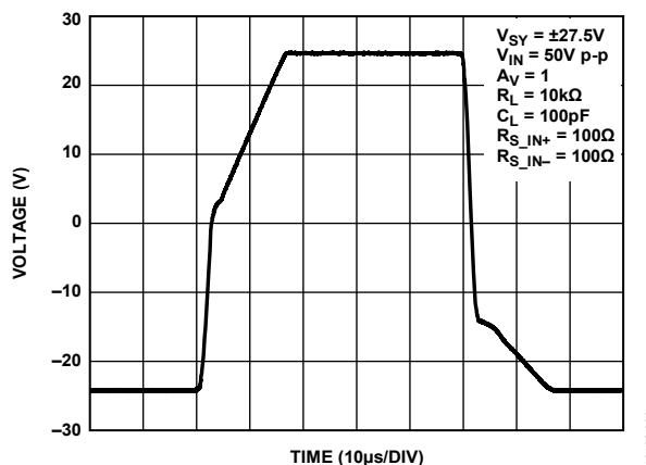
Figure 38. Large Signal Transient Response, V_{SY} = \pm 27.5V
