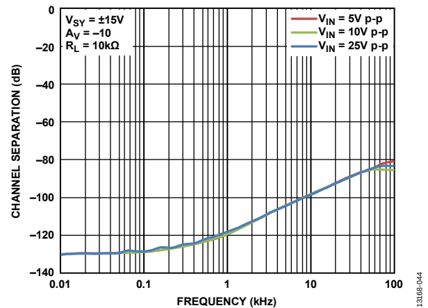
Figure 46. Channel Separation vs. Frequency, V_{SY} = \pm 15\text{ V}
