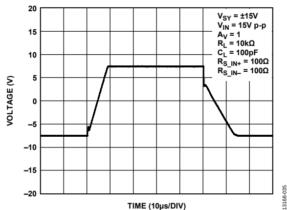
Figure 37. Large Signal Transient Response, V_{SY} = \pm 15V
