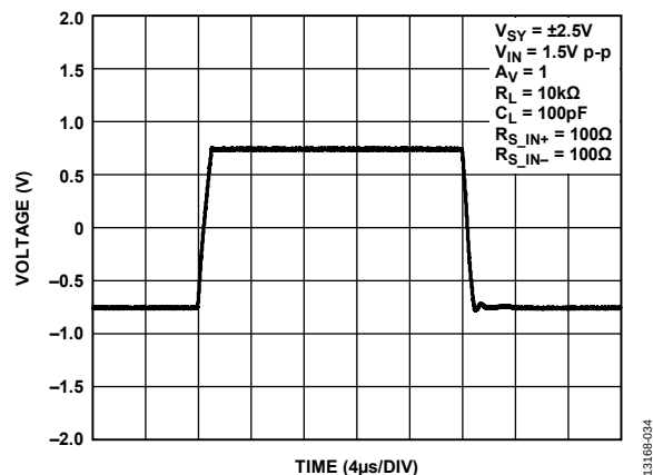
Figure 36. Large Signal Transient Response, V_{SY} = \pm 2.5V
