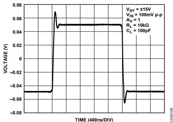
Figure 40. Small Signal Transient Response, V_{SY} = \pm 15V
