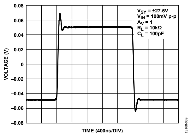
Figure 41. Small Signal Transient Response, V_{SY} = \pm 27.5V
