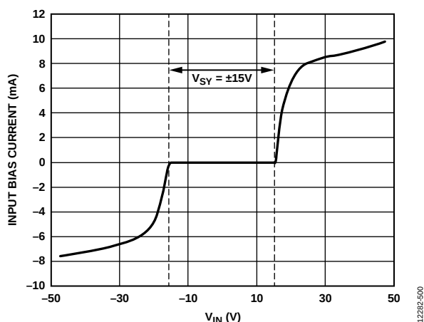
Figure 88. Input Bias Current During Positive and Negative Overvoltage, V_{SY} = \pm 15 V, Voltage Follower Configuration
