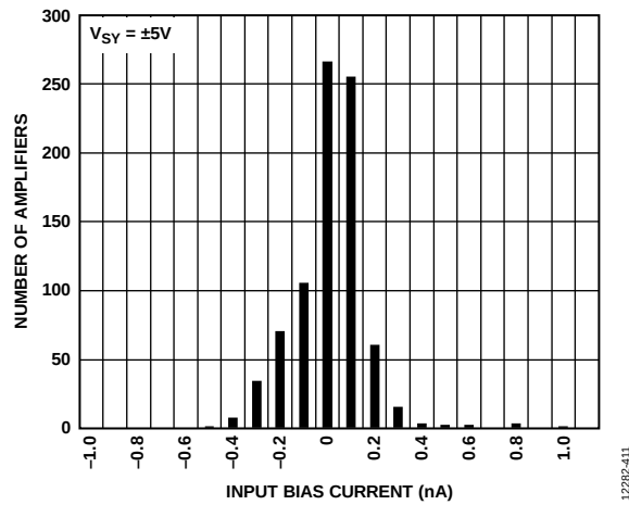
Figure 28. Input Bias Current Distribution, V_{SY} = \pm 5V
