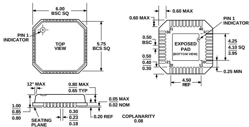
COMPLIANT TO JEDEC STANDARDS MO-220-VJJD-2 Figure 47. 40-Lead Lead Frame Chip Scale Package [LFCSP] 6 mm × 6 mm Body (CP-40) Dimensions shown in millimeters
