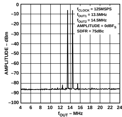
Figure 15. Two-Tone SFDR
