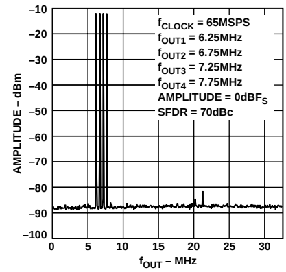
Figure 16. Four-Tone SFDR
