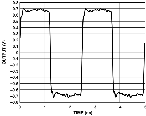
Figure 15. Output Waveform, 21 mA Mode (400 MHz) with 100 Ω Termination at Load
