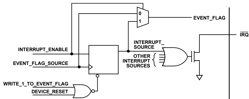
Figure 78. Simplified Schematic of \overline{IRQ} Circuitry
